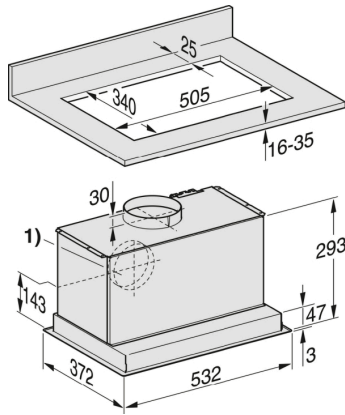
DA 2450, DA 2558 (Installation drawing)
